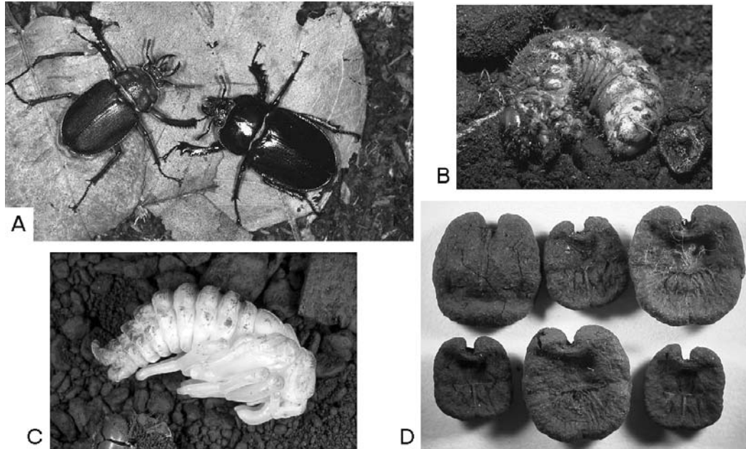
FIG. 5. Sphaenognathus ( Australognathus ) munchowae sp. nov., A, living minor male (left) and female, reared from Consuelo Tableland larvae (photo Gary Cranitch, QM); B, third instar larva from Consuelo Tableland (photo Steve Wilson); C, male pupa, lateral view (photo Paul Zborowski); D, faecal pellets of second (small) and third (large) instar larvae.
